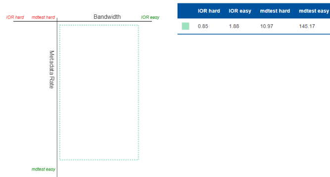
Fig. 3. Single run of POSIX-IO IO500 plotted into Cartesian coordinate system made of the aggregated read-write bandwidth score and metadata score
